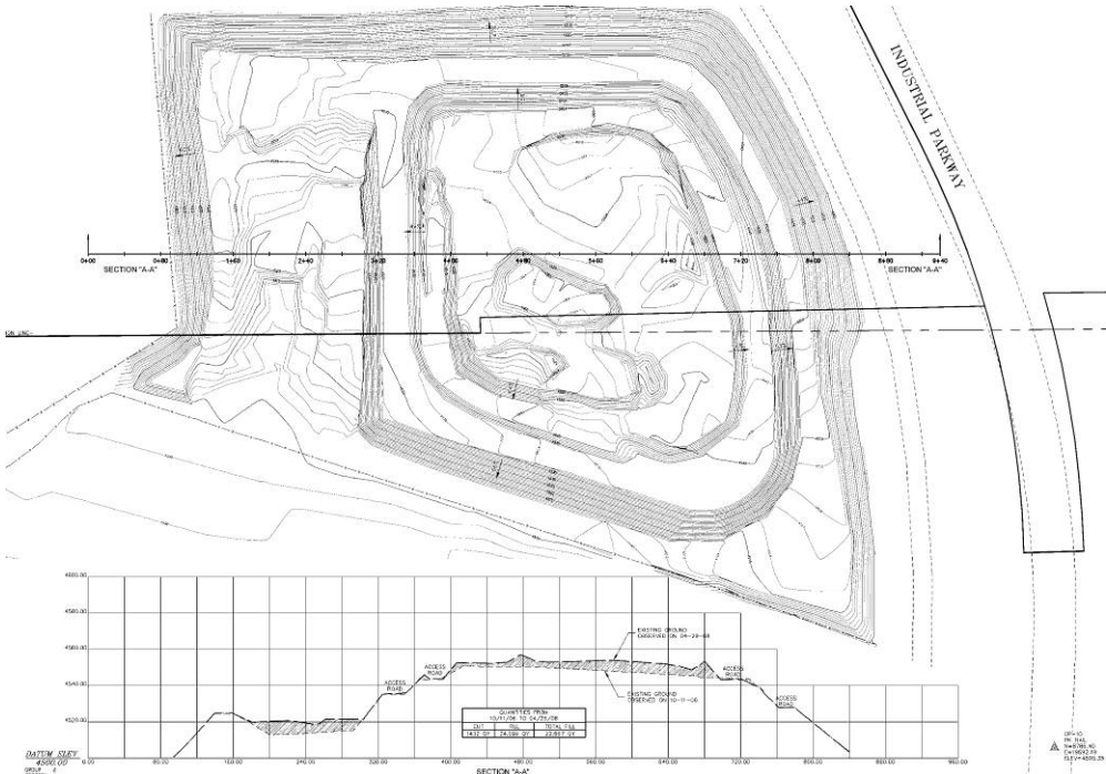
A section exhibit showing cut and fill quantities through the existing PSP landfill
